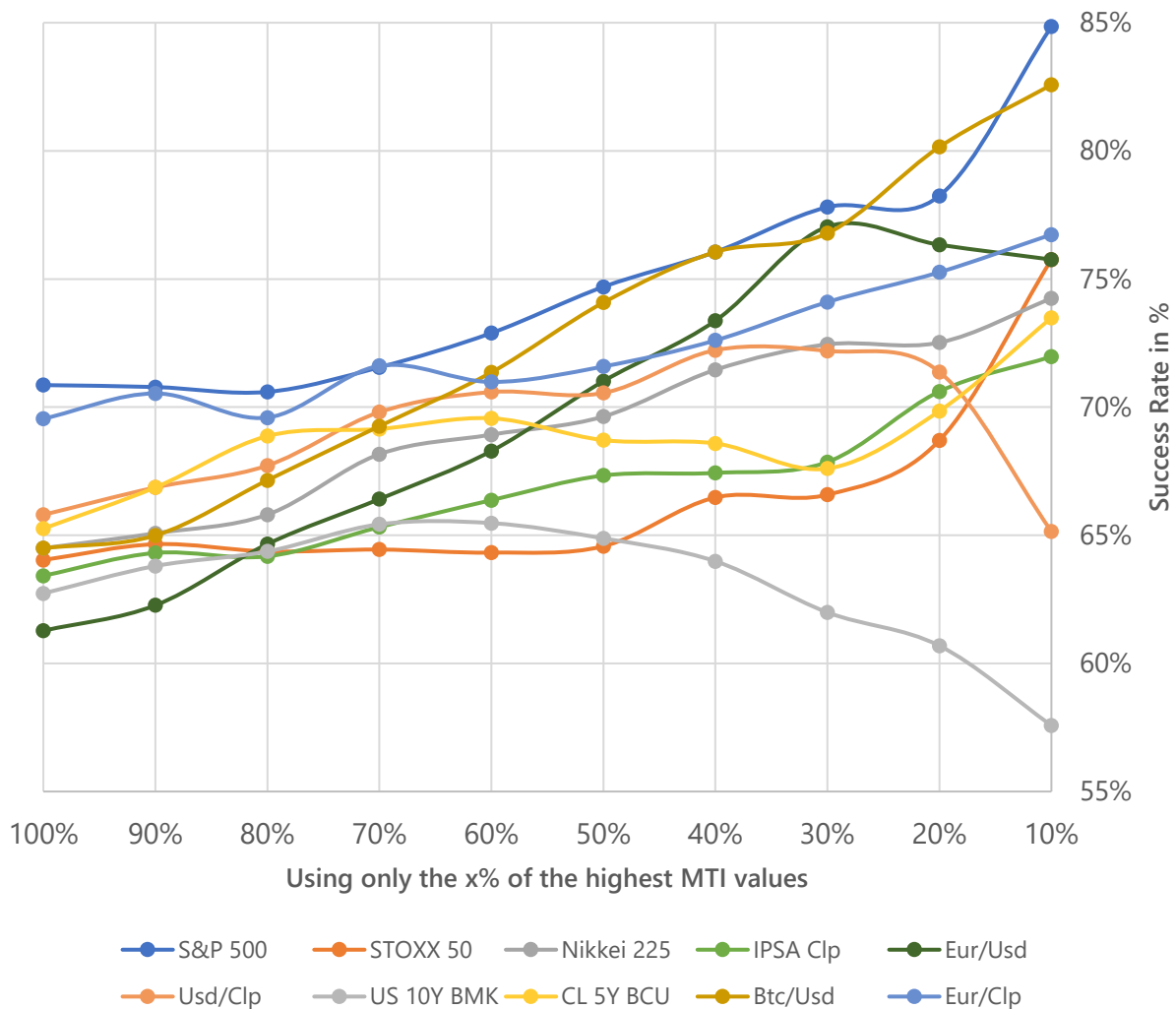
Success Rate vs % of the time
